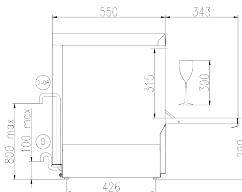
Rear side
