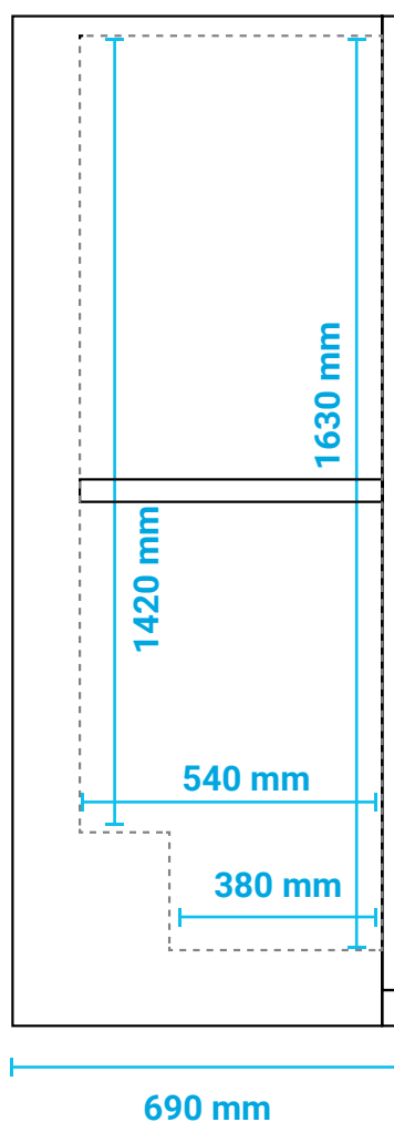
SIDE
